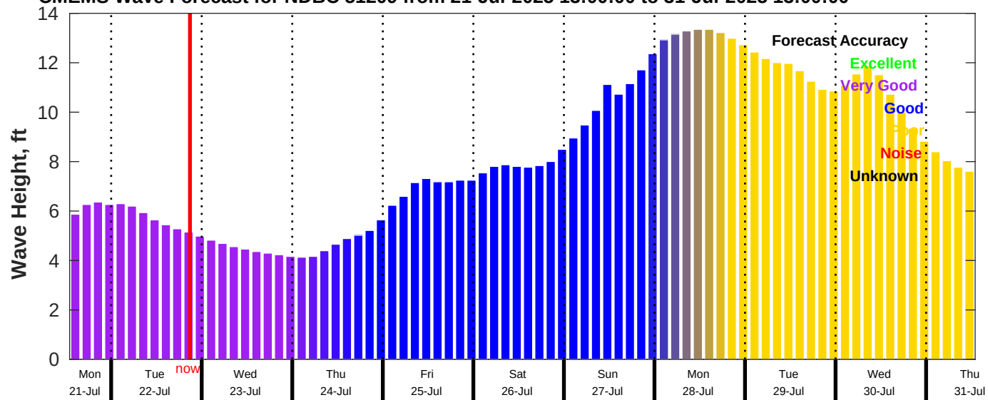
CMEMS Wave Forecast for NDBC 51209 from 21-Jul-2025 13:00:00 to 31-Jul-2025 13:00:00
