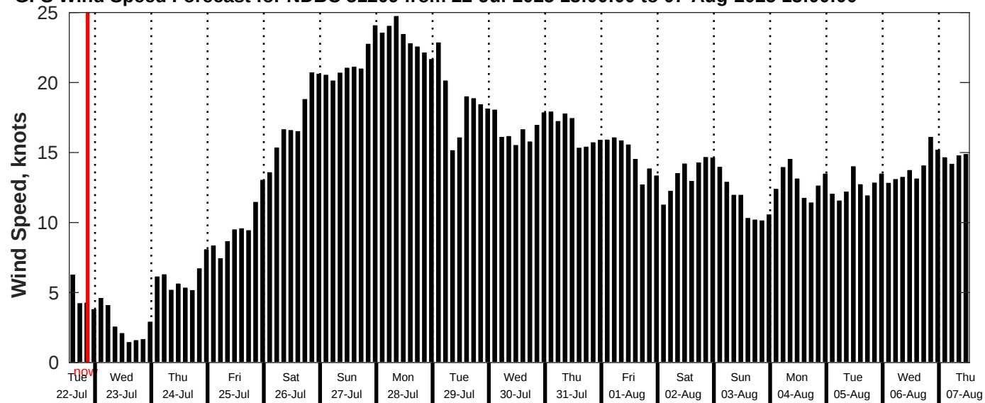
GFS Wind Speed Forecast for NDBC 51209 from 22-Jul-2025 13:00:00 to 07-Aug-2025 13:00:00
