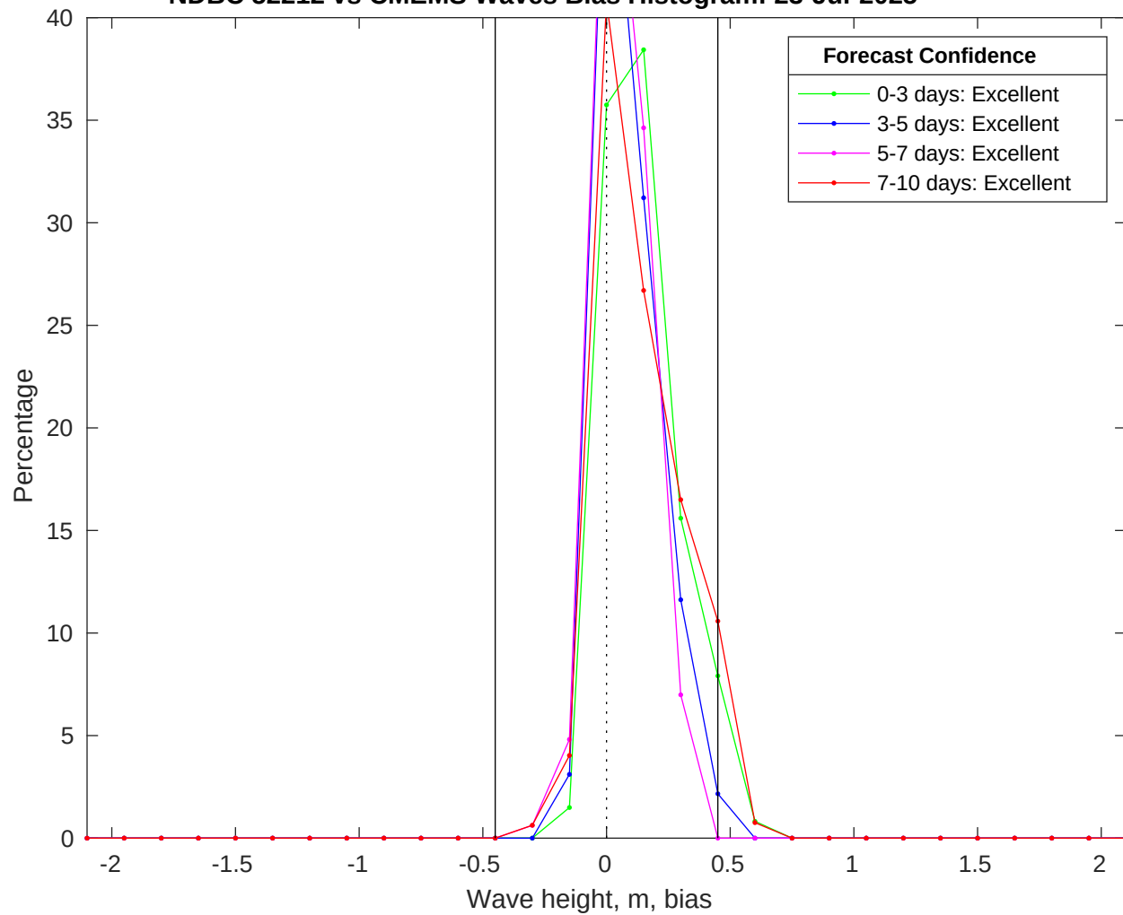
NDBC 52212 vs CMEMS Waves Bias Histogram: 23-Jul-2025
