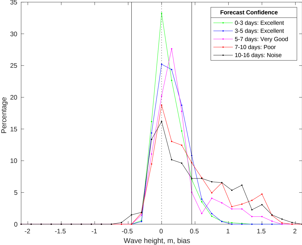
NDBC 52212 vs GFS Waves Bias Histogram: 23-Jul-2025
