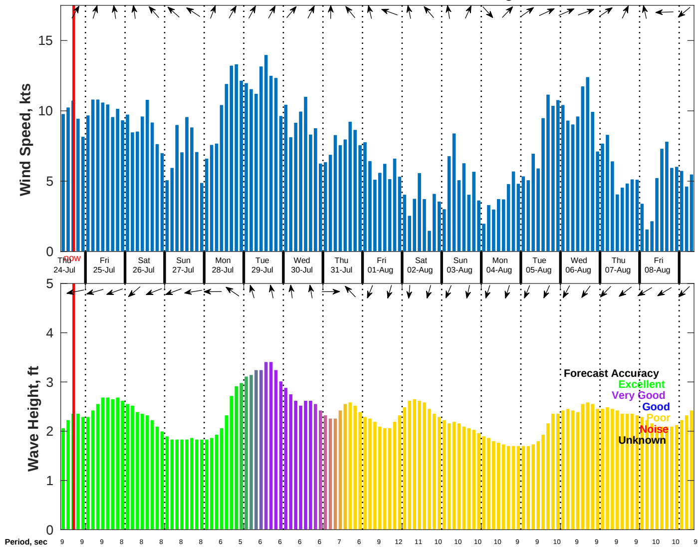
Wind & Wave Forecast for NDBC 52212 from 23-Jul-2025 09:00:00 to 08-Aug-2025 09:00:00
