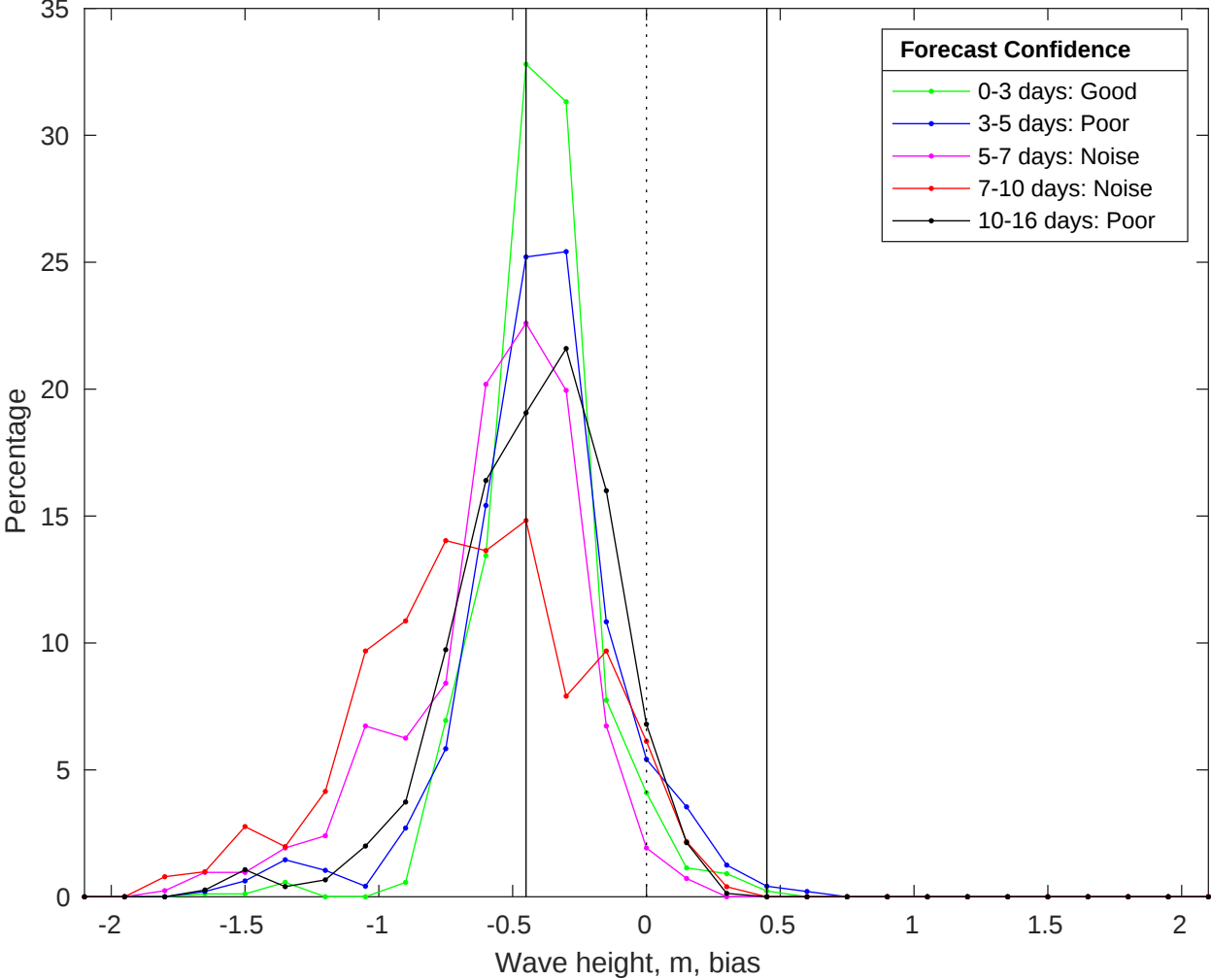
NDBC 52213 vs GFS Waves Bias Histogram: 23-Jul-2025
