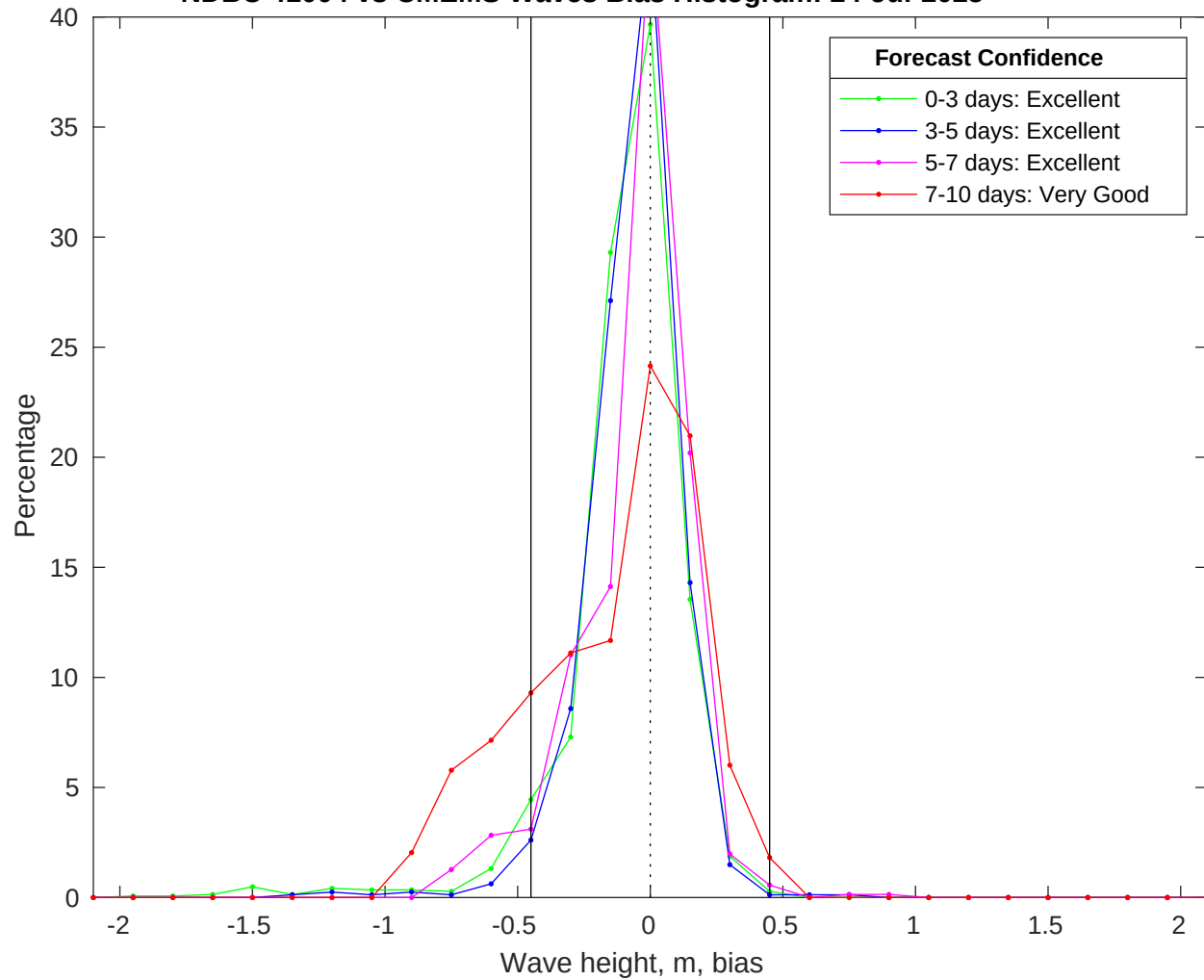
NDBC 41004 vs CMEMS Waves Bias Histogram: 24-Jul-2025
