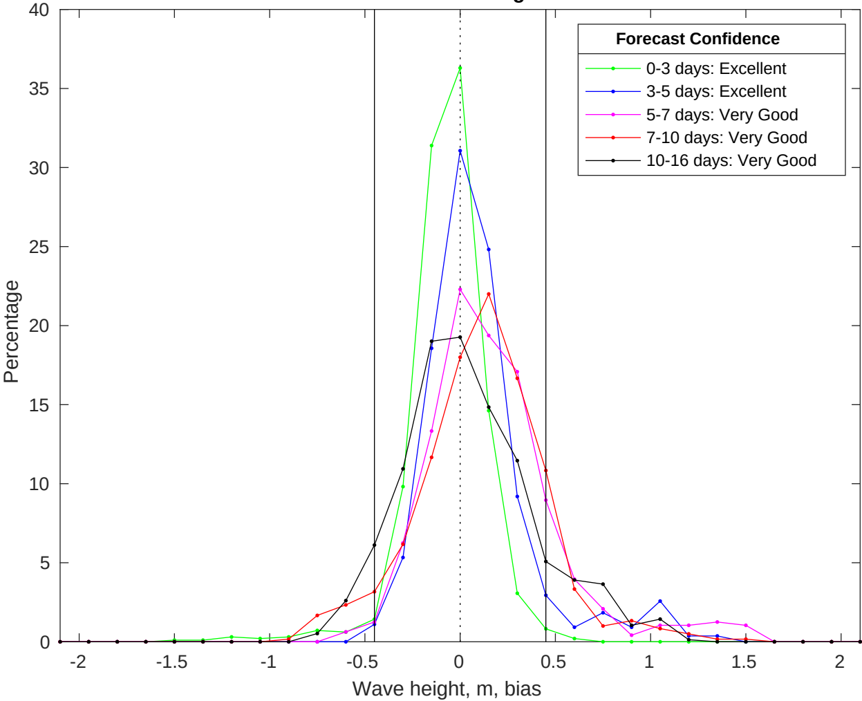
NDBC 41004 vs GFS Waves Bias Histogram: 24-Jul-2025
