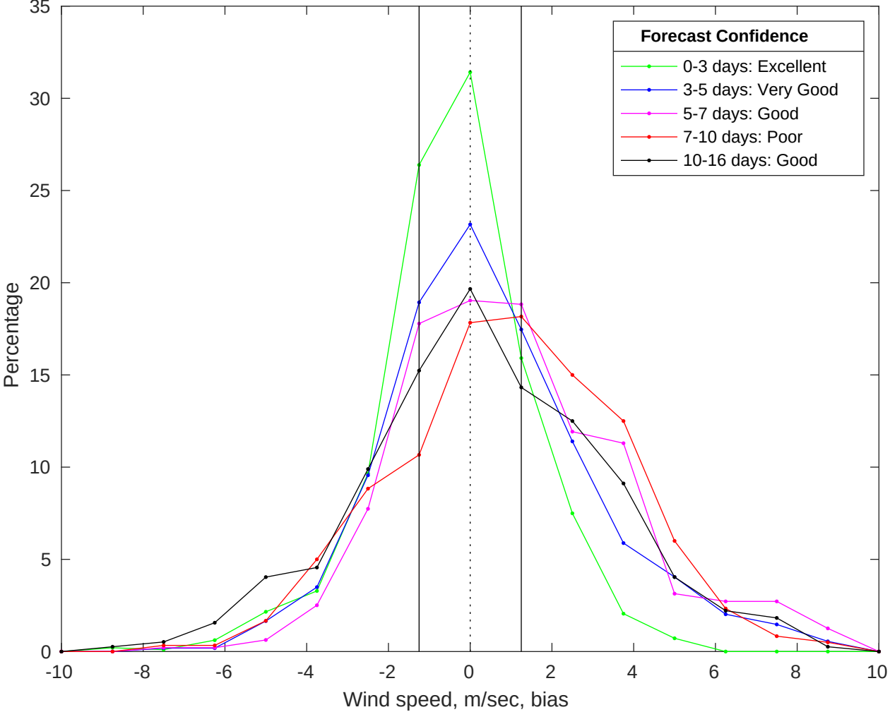
NDBC 41004 vs GFS Winds Bias Histogram: 24-Jul-2025
