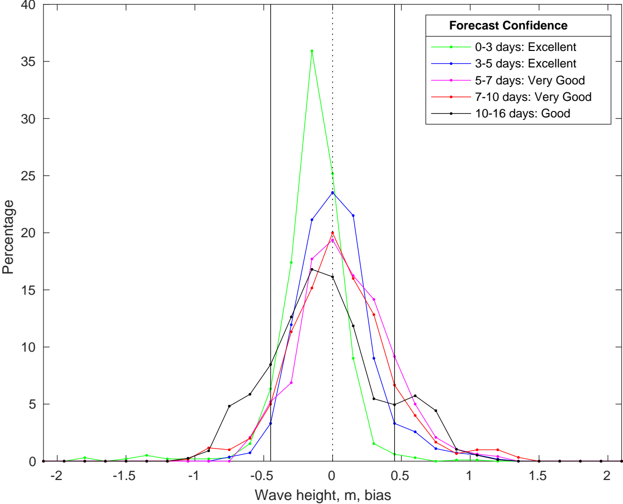
NDBC 41013 vs GFS Waves Bias Histogram: 24-Jul-2025
