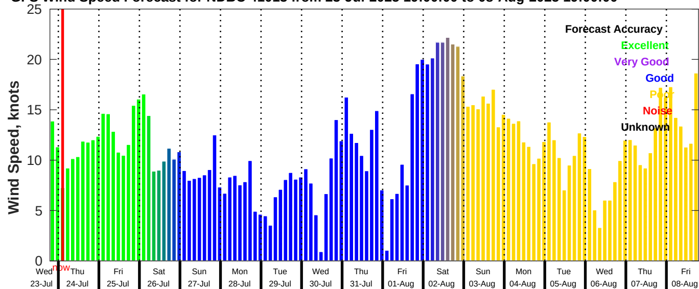
GFS Wind Speed Forecast for NDBC 41013 from 23-Jul-2025 19:00:00 to 08-Aug-2025 19:00:00
