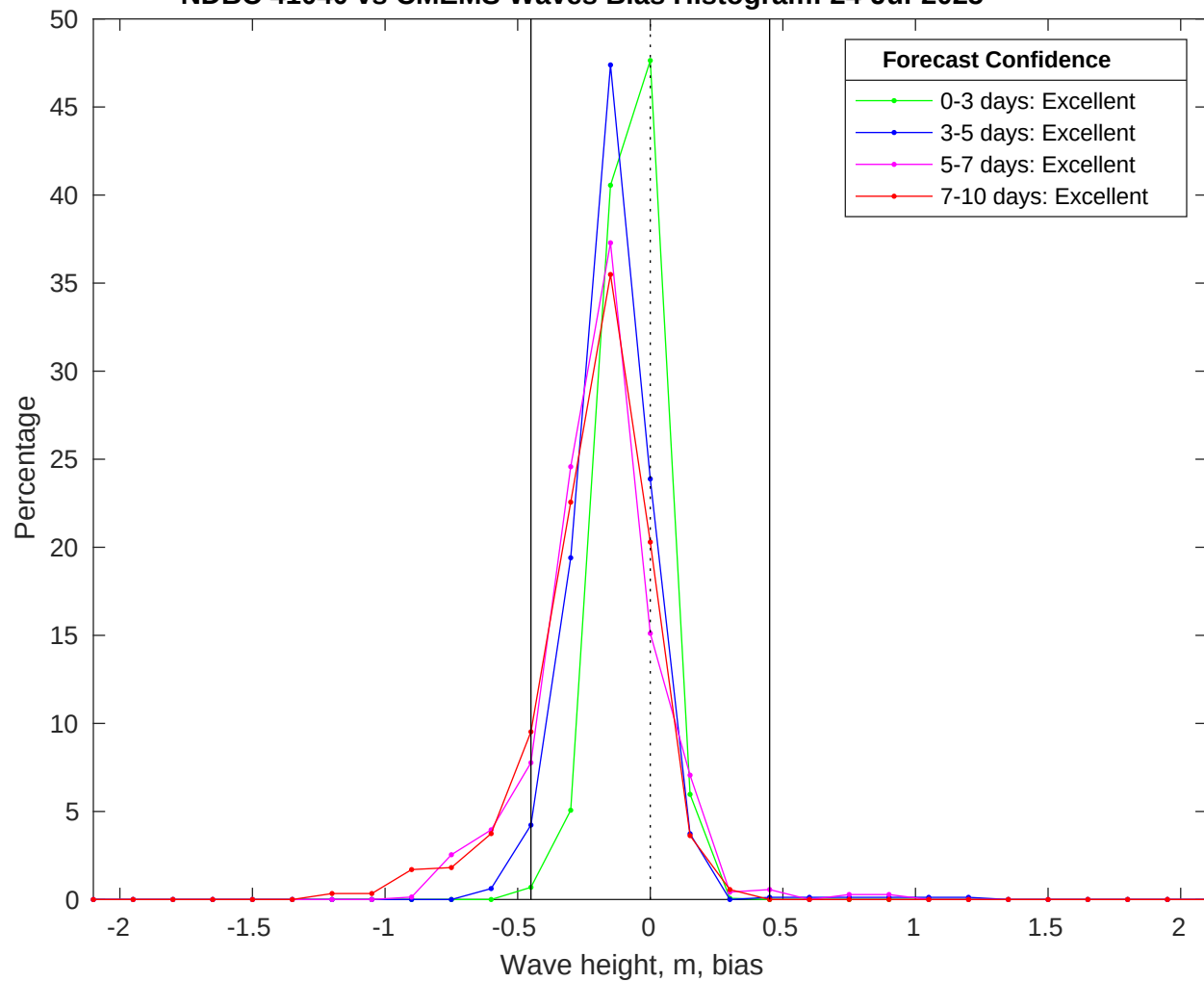
NDBC 41040 vs CMEMS Waves Bias Histogram: 24-Jul-2025
