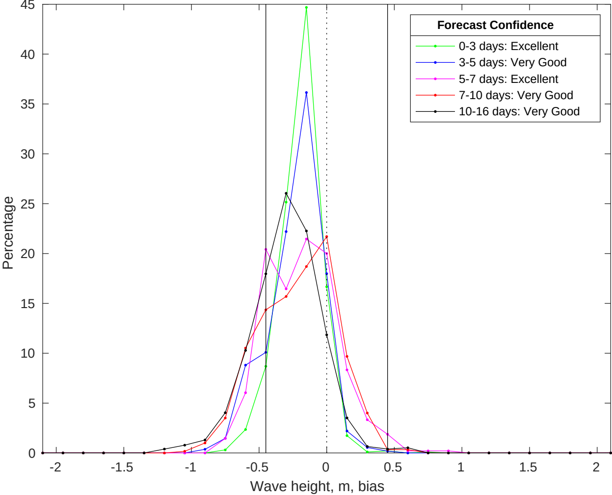
NDBC 41040 vs GFS Waves Bias Histogram: 24-Jul-2025
