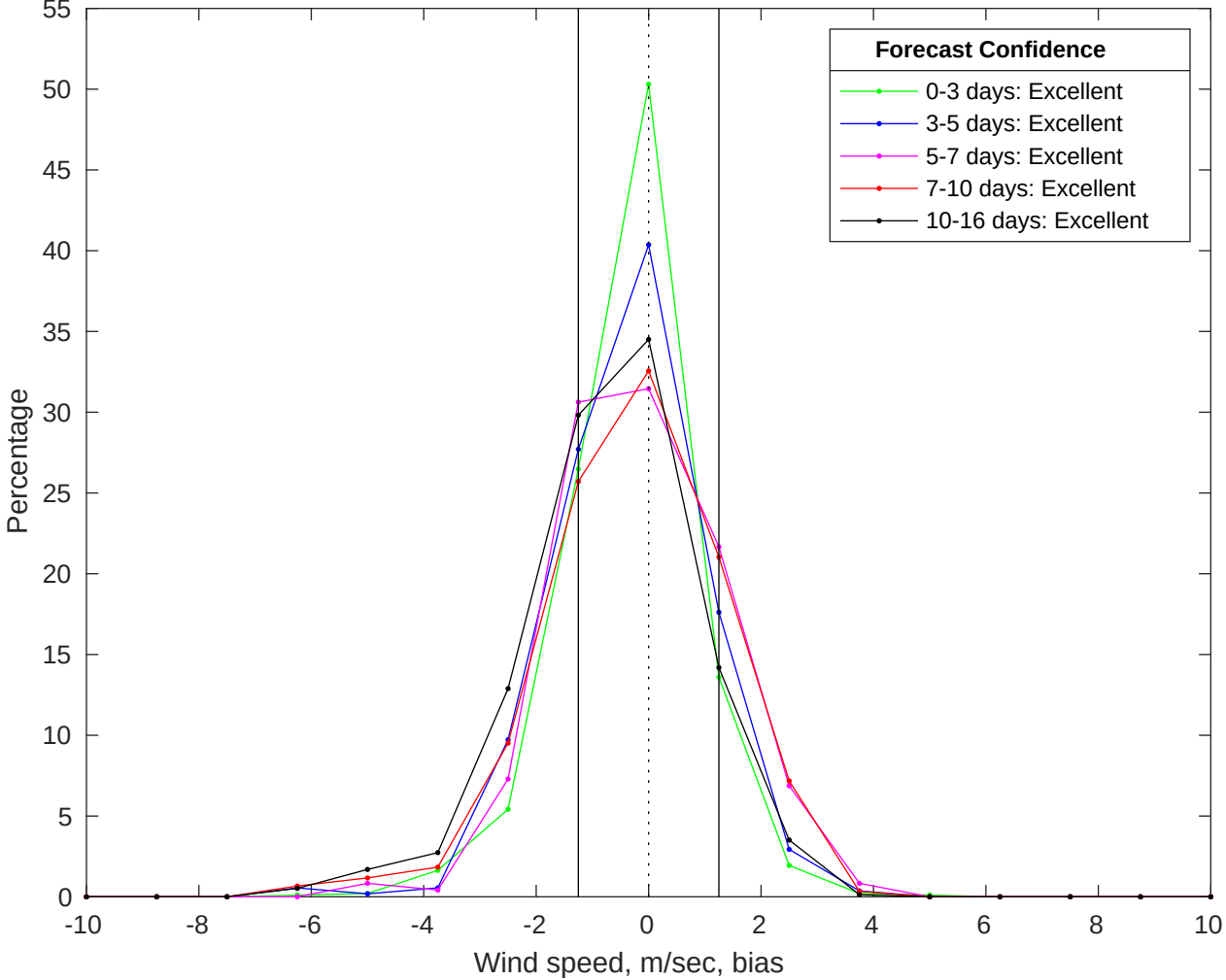
NDBC 41040 vs GFS Winds Bias Histogram: 24-Jul-2025
