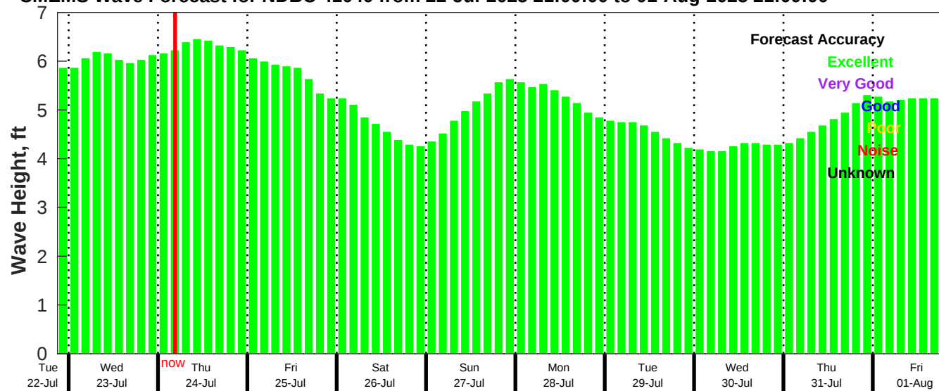
CMEMS Wave Forecast for NDBC 41040 from 22-Jul-2025 21:00:00 to 01-Aug-2025 21:00:00
