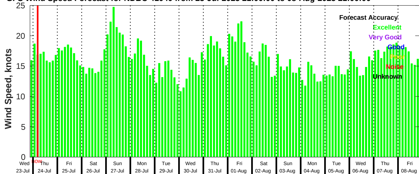
GFS Wind Speed Forecast for NDBC 41040 from 23-Jul-2025 21:00:00 to 08-Aug-2025 21:00:00
