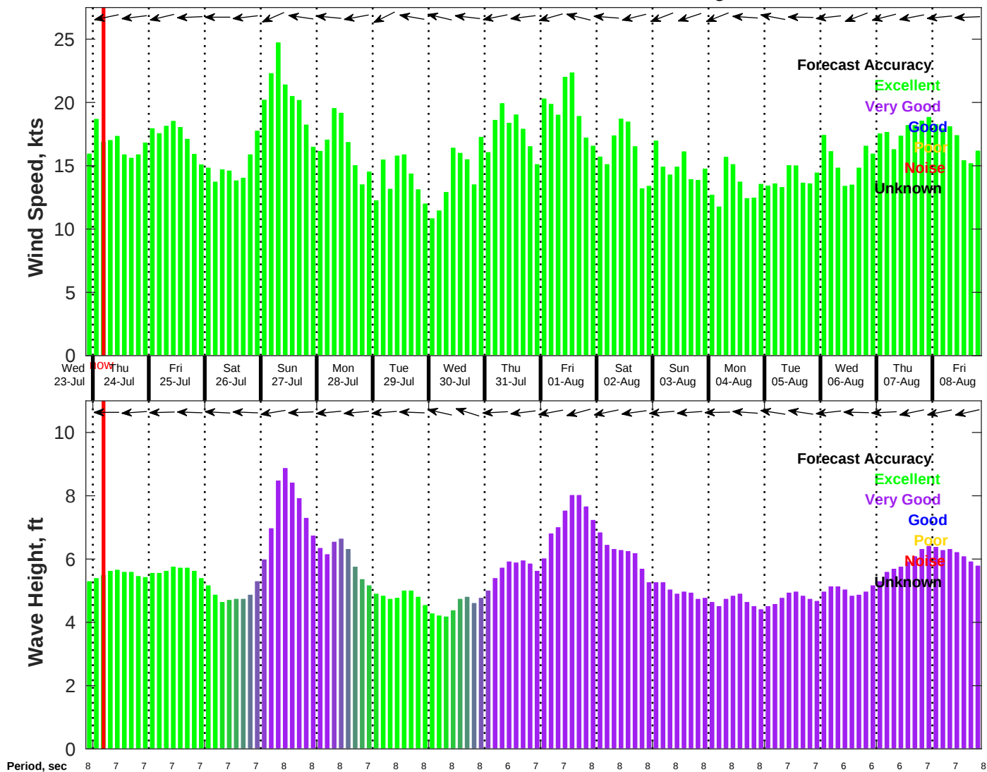
Wind & Wave Forecast for NDBC 41040 from 23-Jul-2025 21:00:00 to 08-Aug-2025 21:00:00
