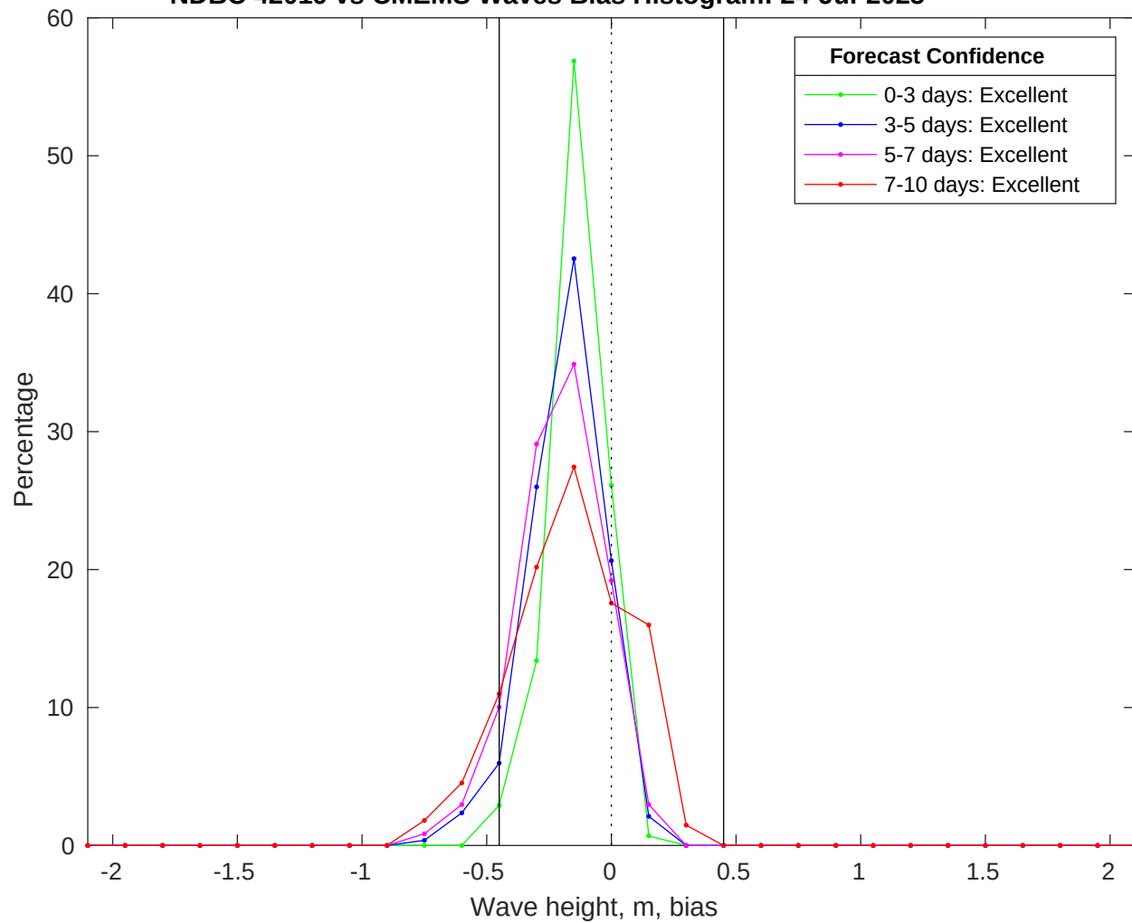
NDBC 42019 vs CMEMS Waves Bias Histogram: 24-Jul-2025
