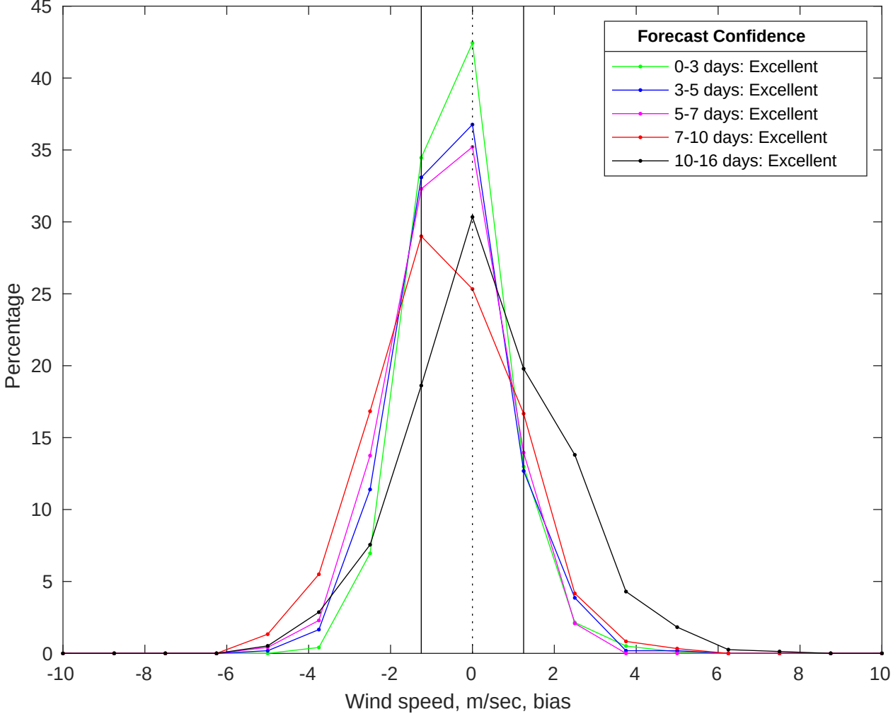
NDBC 42019 vs GFS Winds Bias Histogram: 24-Jul-2025
