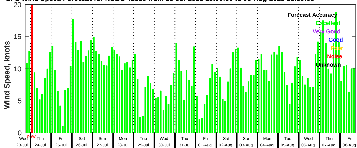
GFS Wind Speed Forecast for NDBC 42020 from 23-Jul-2025 18:00:00 to 08-Aug-2025 18:00:00
