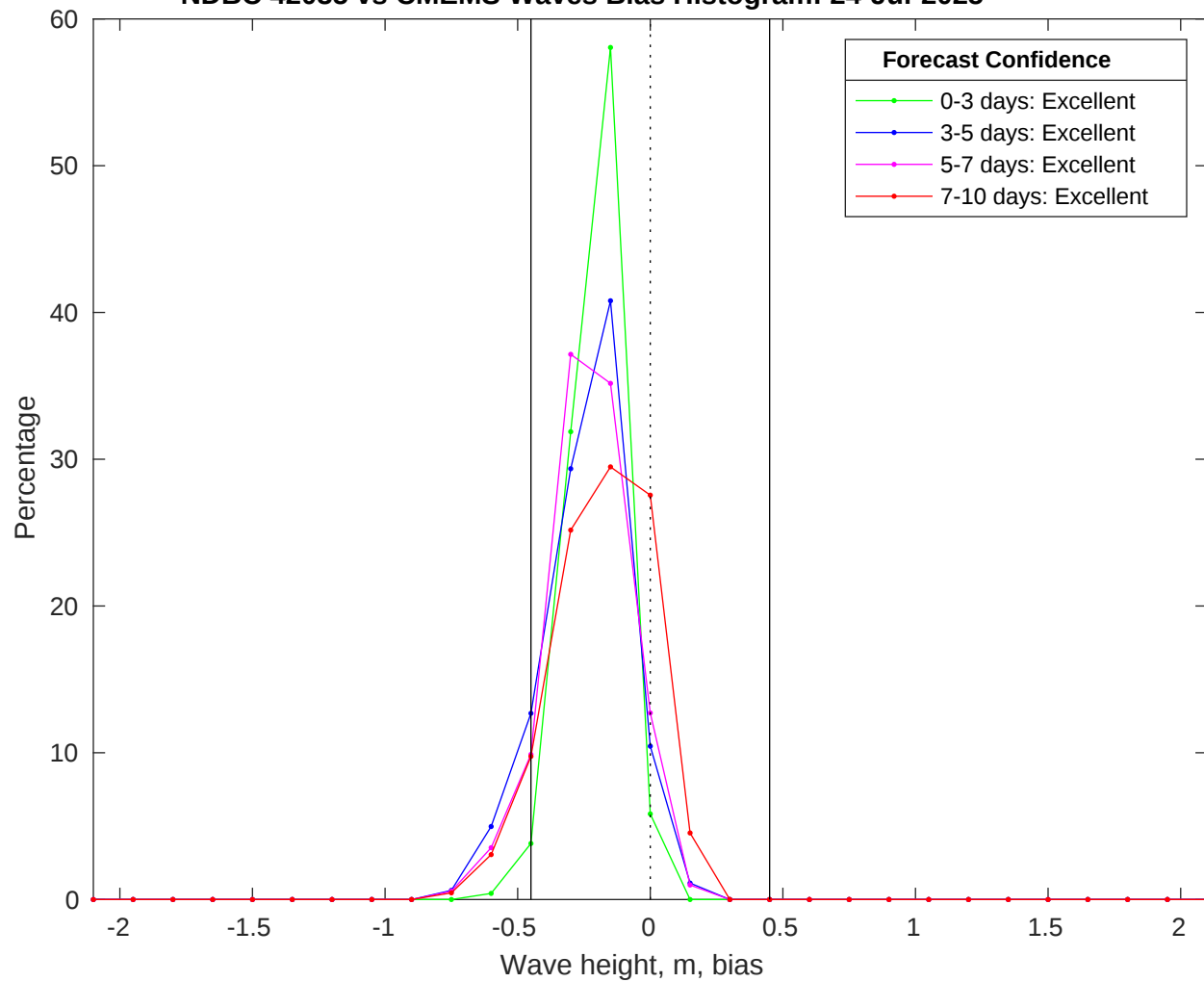
NDBC 42035 vs CMEMS Waves Bias Histogram: 24-Jul-2025
