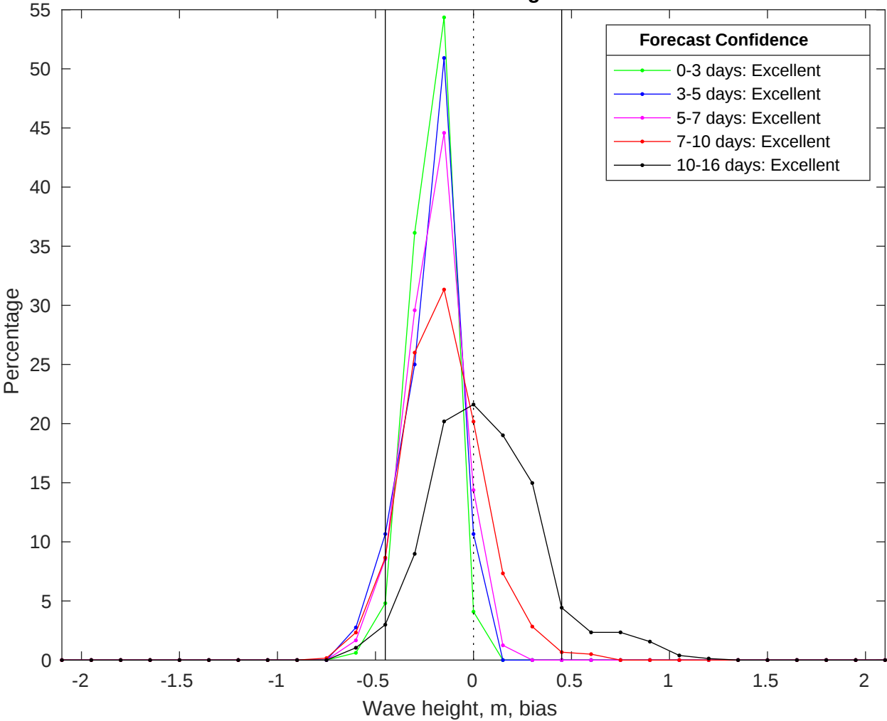
NDBC 42035 vs GFS Waves Bias Histogram: 24-Jul-2025
