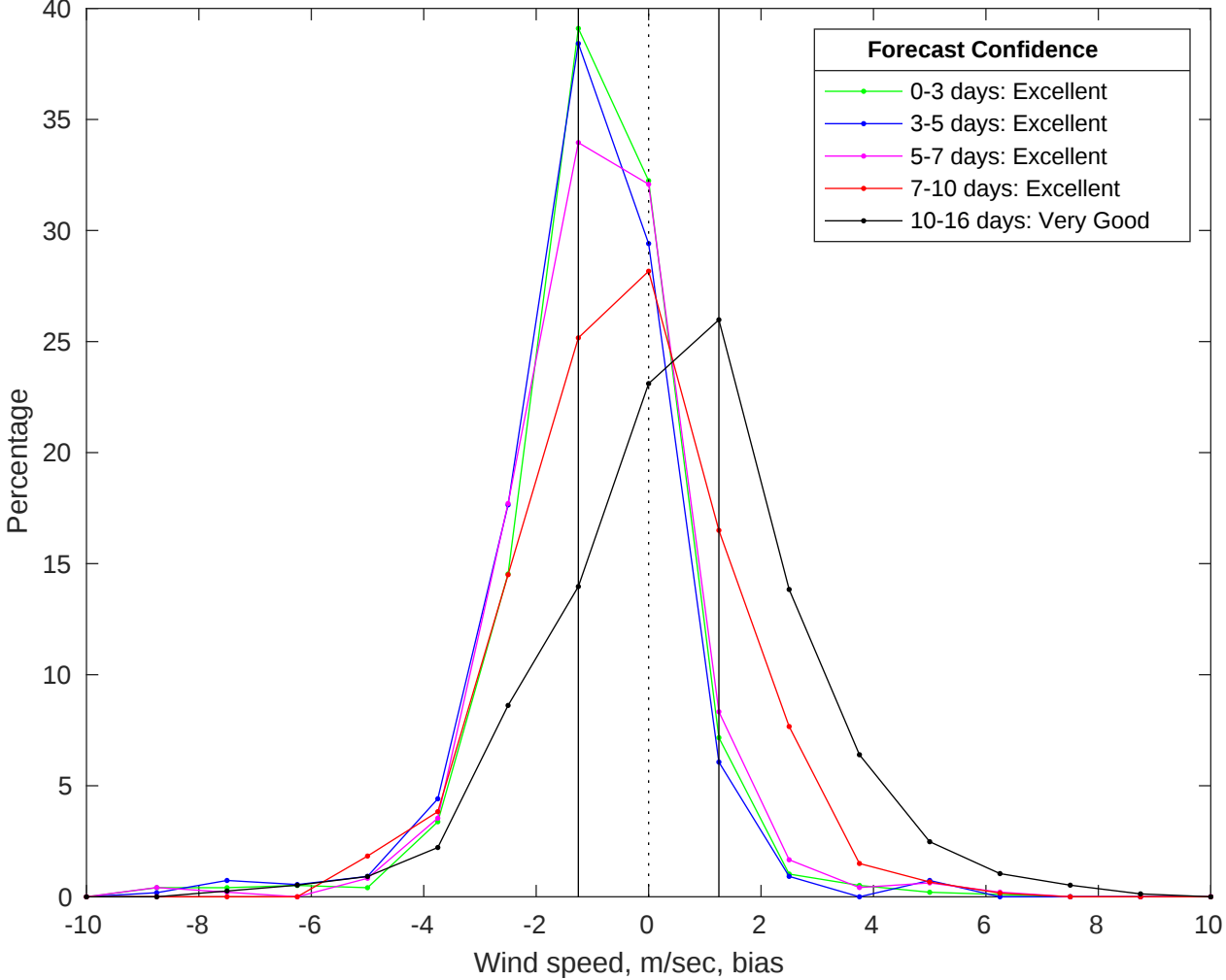
NDBC 42035 vs GFS Winds Bias Histogram: 24-Jul-2025
