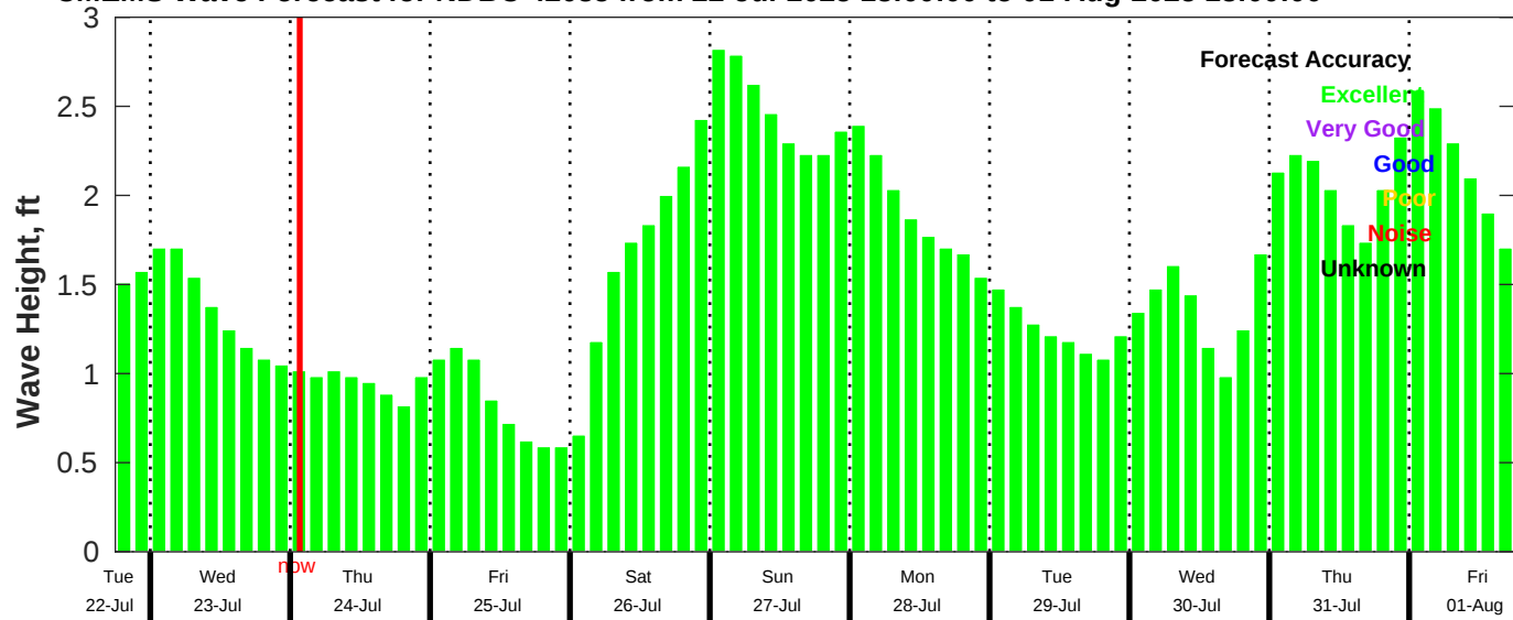
CMEMS Wave Forecast for NDBC 42035 from 22-Jul-2025 18:00:00 to 01-Aug-2025 18:00:00
