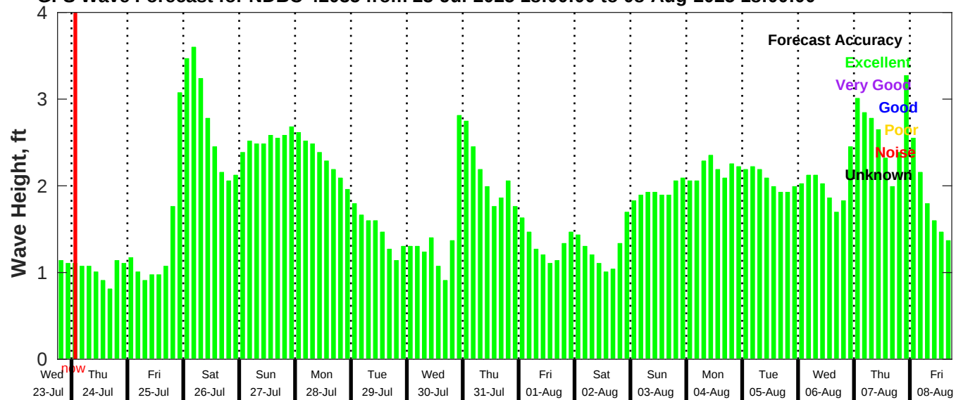
GFS Wave Forecast for NDBC 42035 from 23-Jul-2025 18:00:00 to 08-Aug-2025 18:00:00
