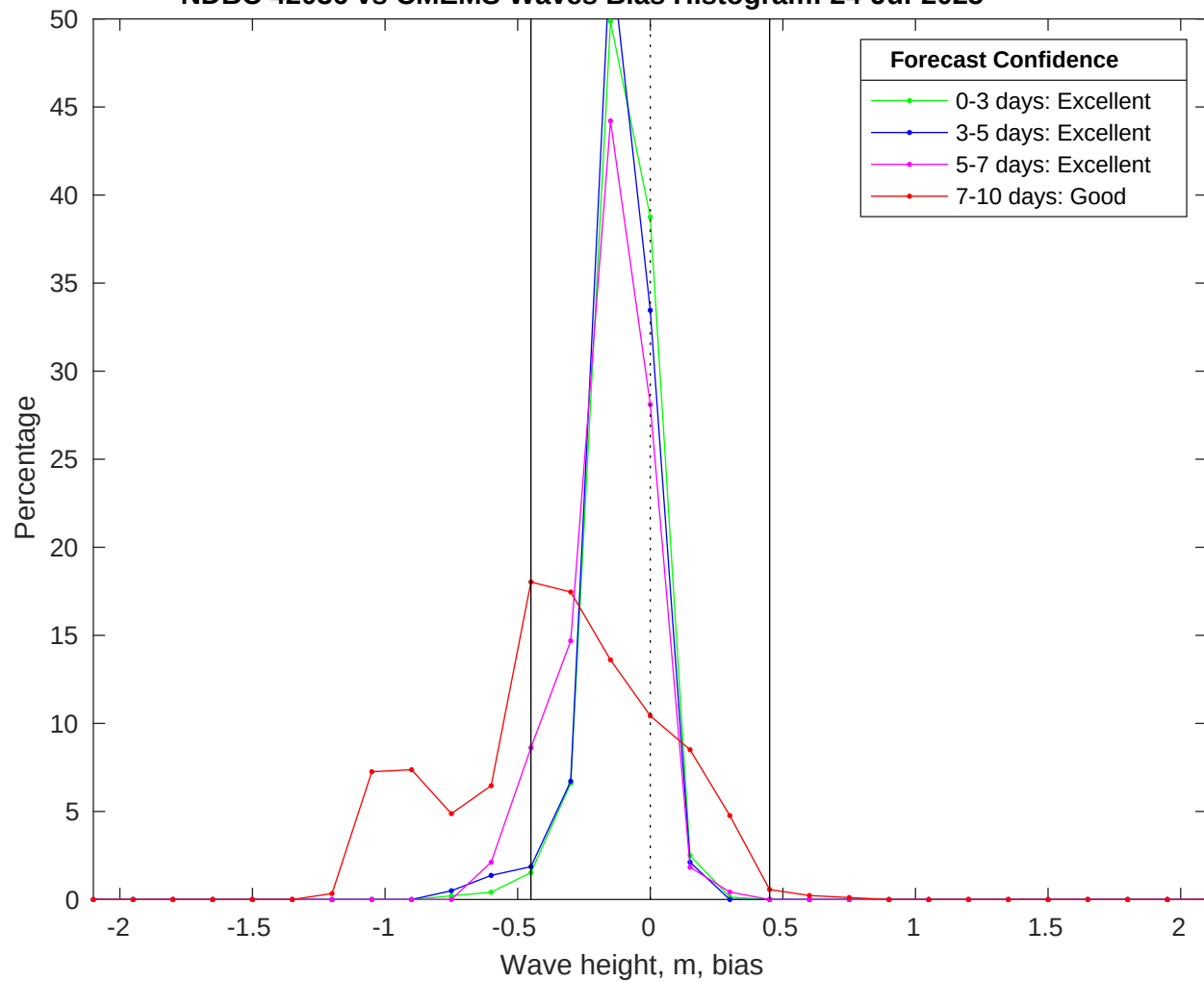
NDBC 42036 vs CMEMS Waves Bias Histogram: 24-Jul-2025
