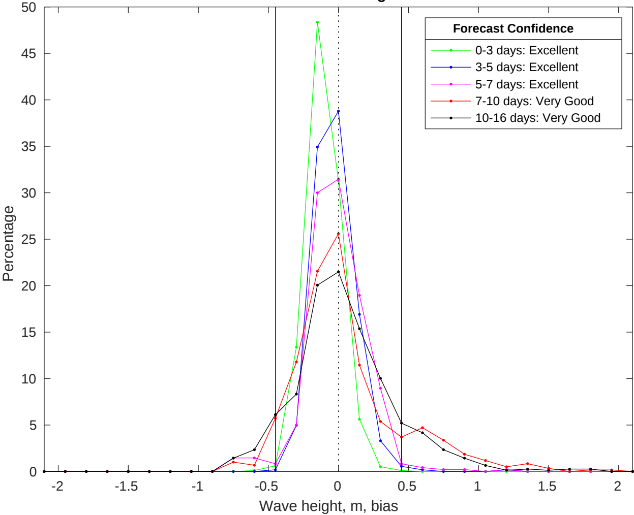
NDBC 42036 vs GFS Waves Bias Histogram: 24-Jul-2025
