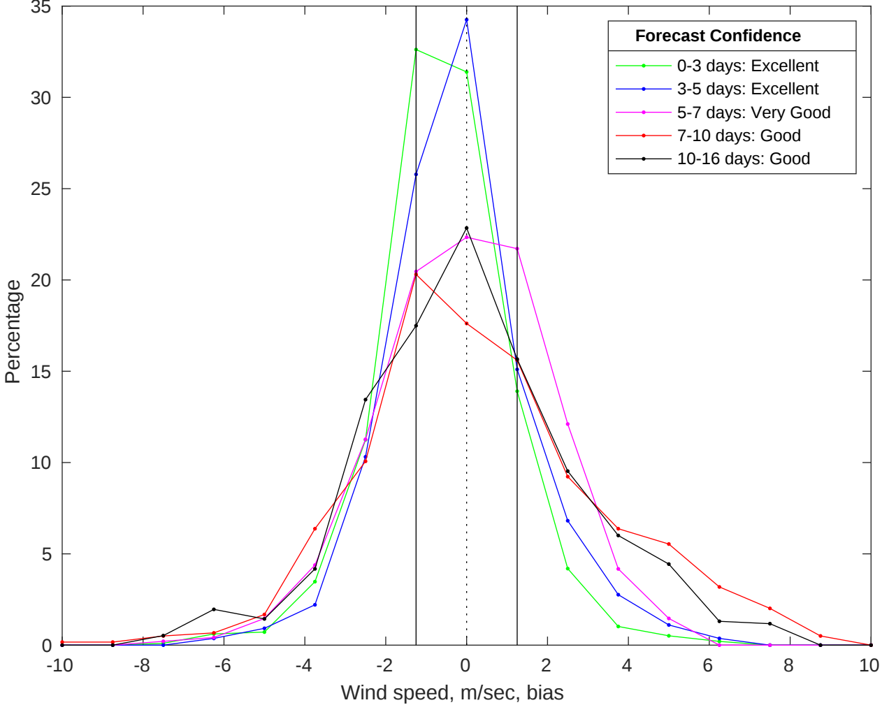
NDBC 42036 vs GFS Winds Bias Histogram: 24-Jul-2025
