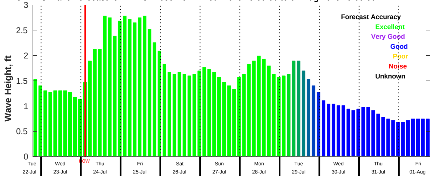
CMEMS Wave Forecast for NDBC 42036 from 22-Jul-2025 19:00:00 to 01-Aug-2025 19:00:00
