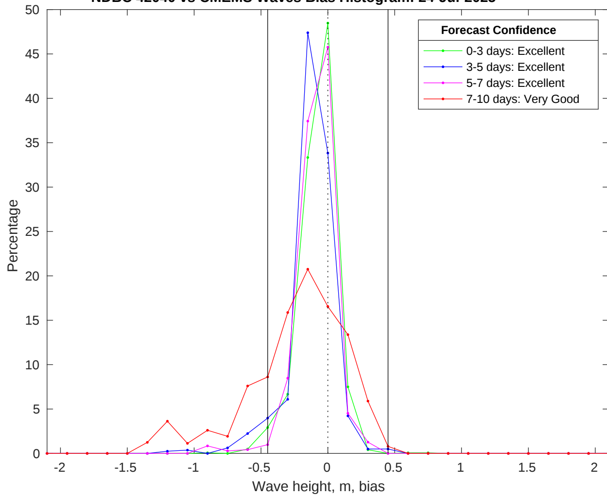
NDBC 42040 vs CMEMS Waves Bias Histogram: 24-Jul-2025
