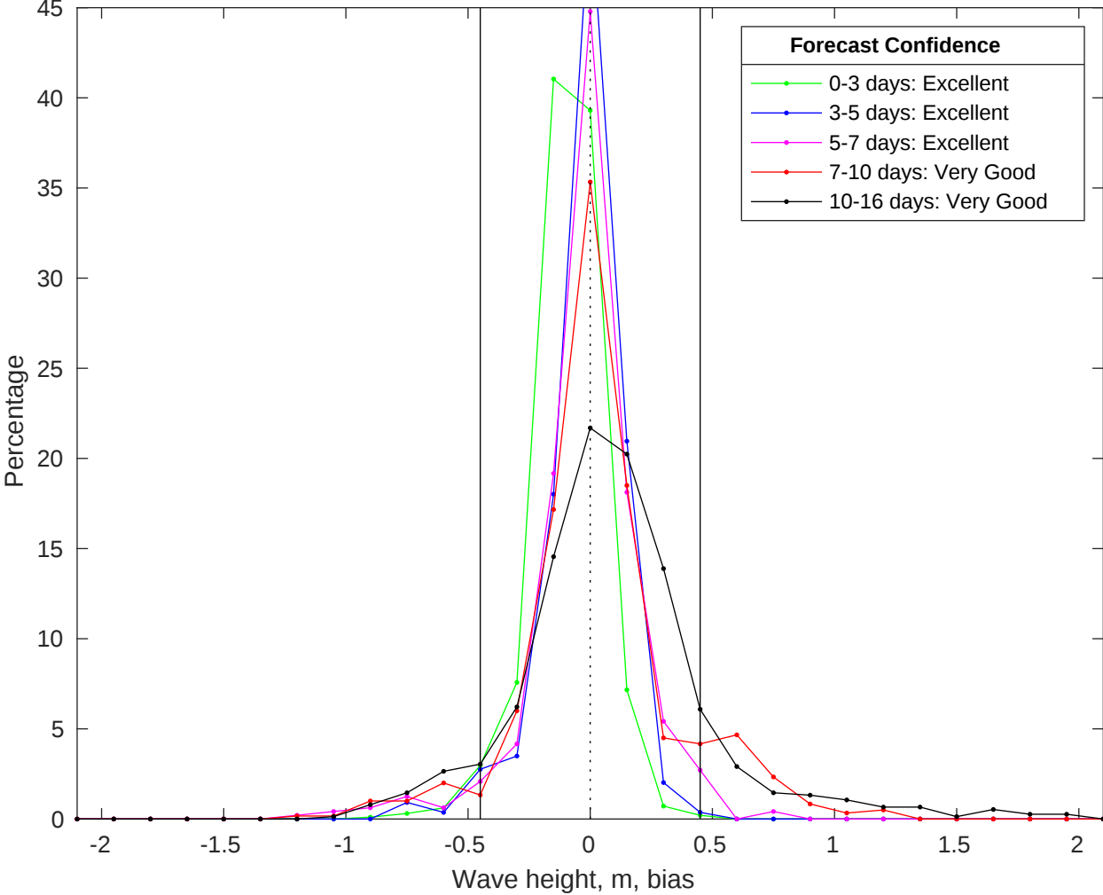
NDBC 42040 vs GFS Waves Bias Histogram: 24-Jul-2025
