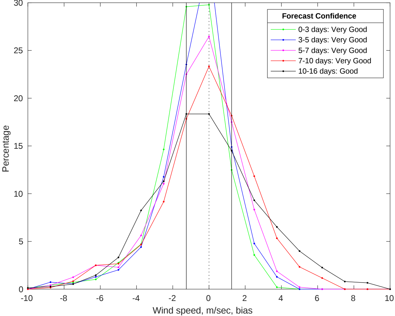
NDBC 42040 vs GFS Winds Bias Histogram: 24-Jul-2025
