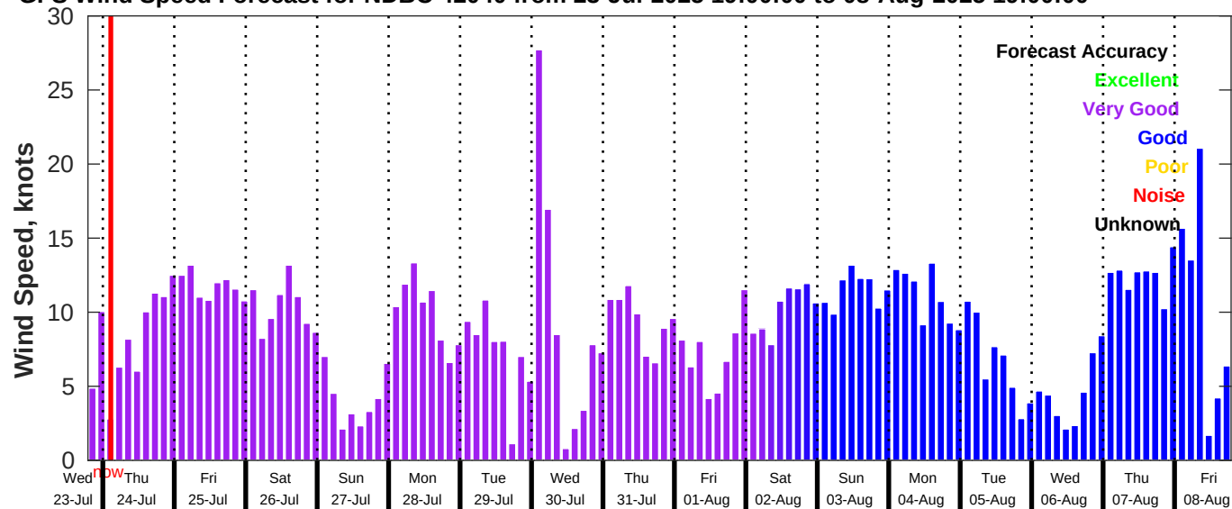
GFS Wind Speed Forecast for NDBC 42040 from 23-Jul-2025 19:00:00 to 08-Aug-2025 19:00:00
