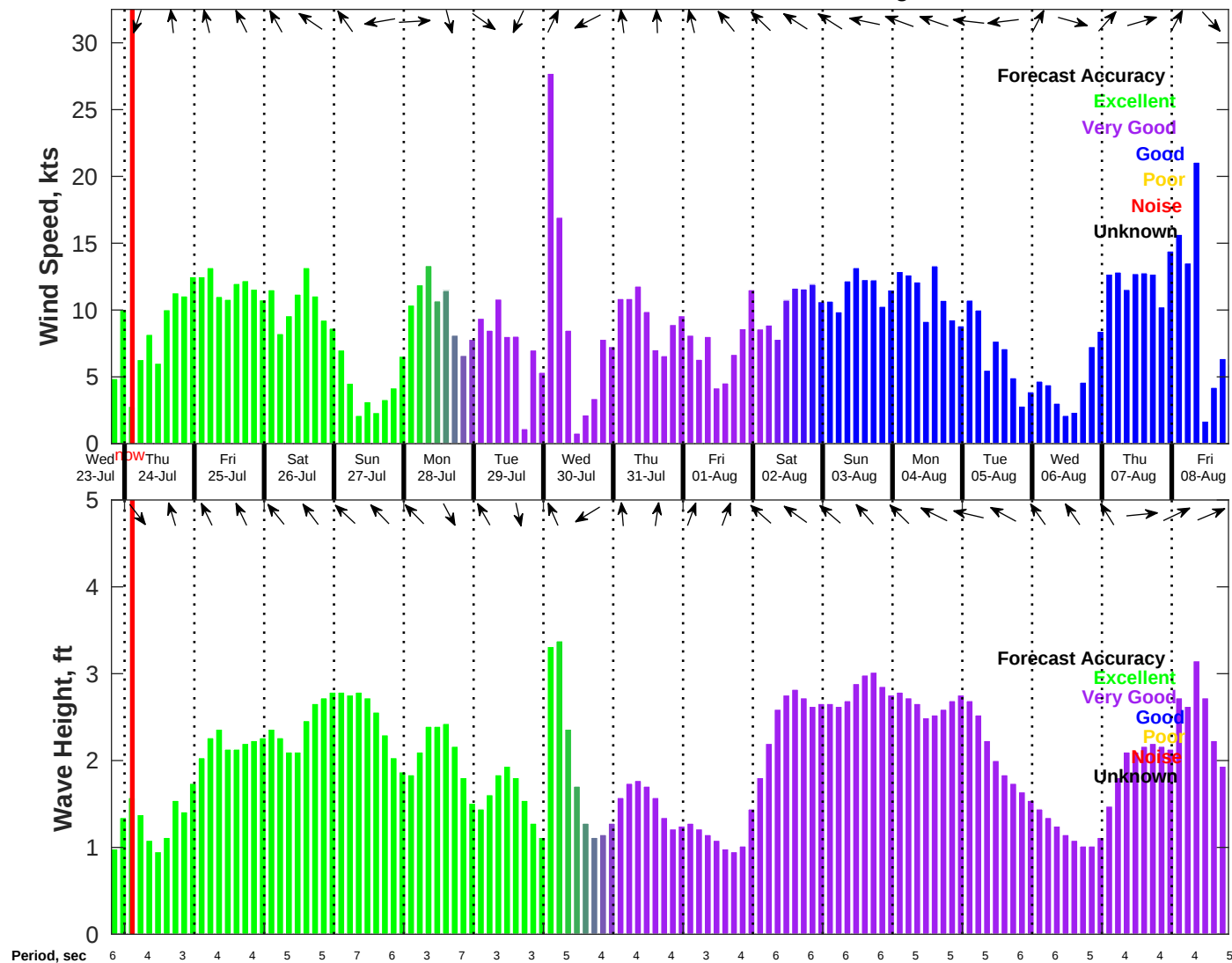
Wind & Wave Forecast for NDBC 42040 from 23-Jul-2025 19:00:00 to 08-Aug-2025 19:00:00
