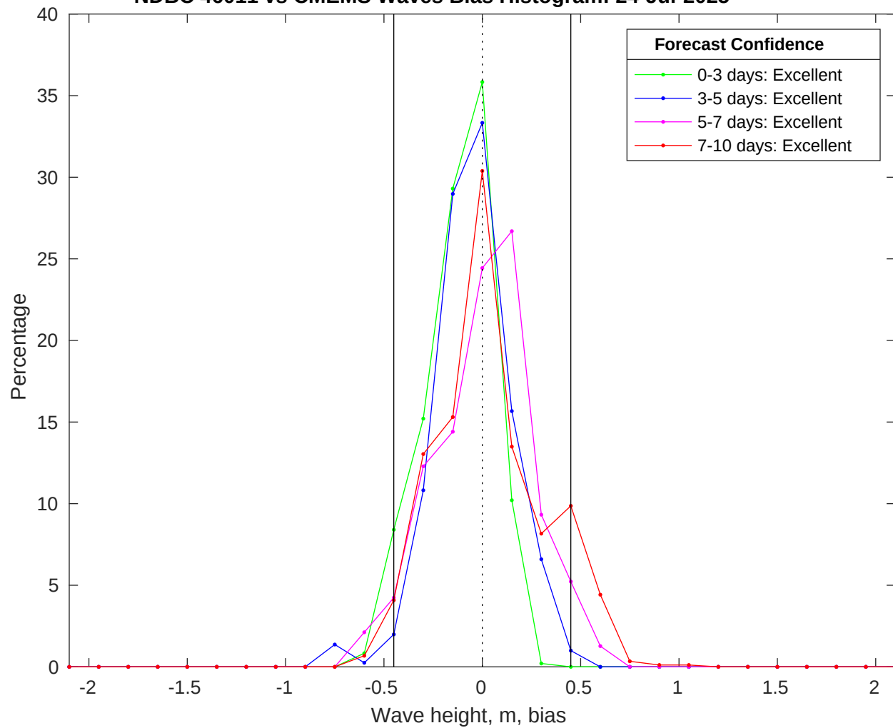
NDBC 46011 vs CMEMS Waves Bias Histogram: 24-Jul-2025
