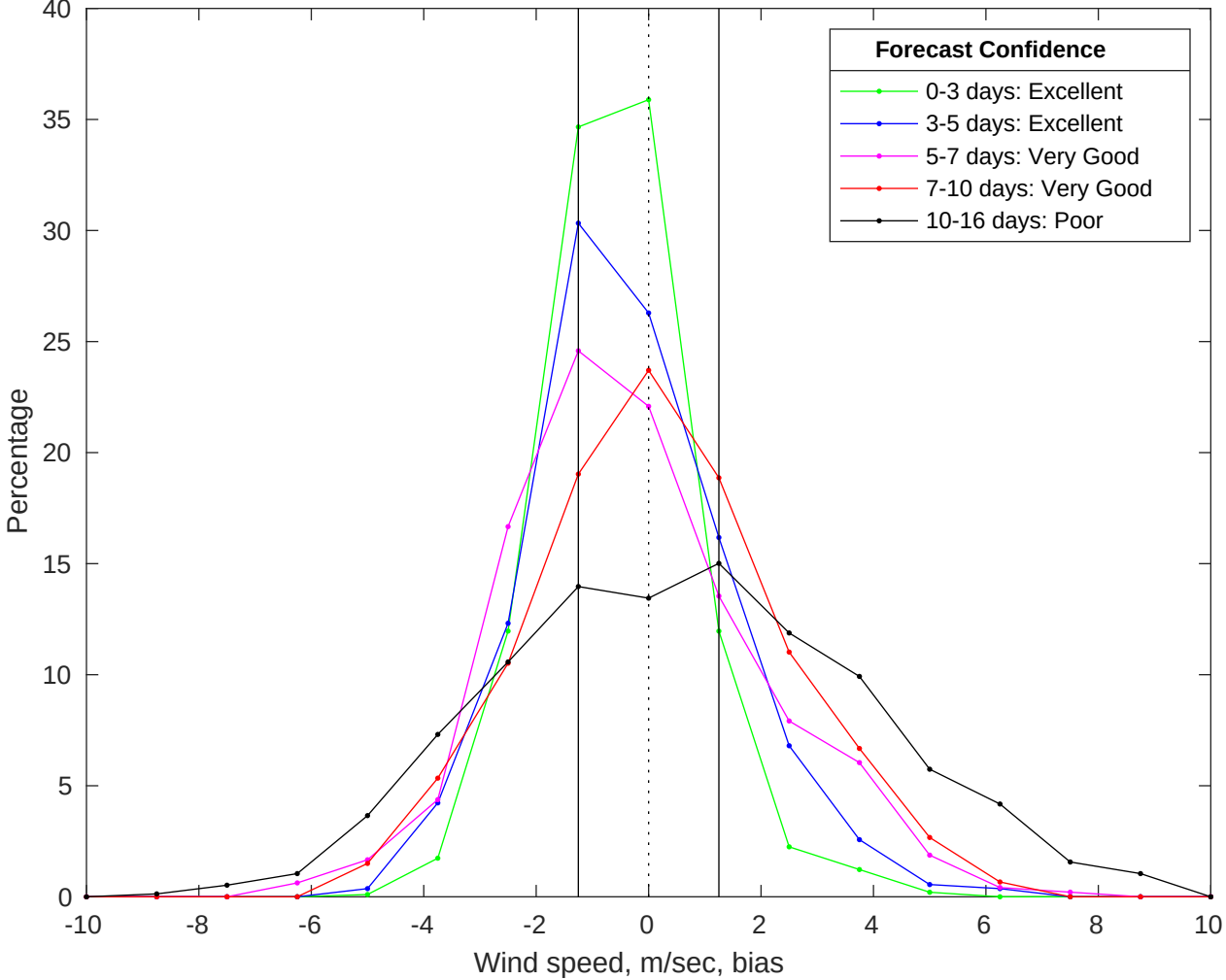
NDBC 46011 vs GFS Winds Bias Histogram: 24-Jul-2025
