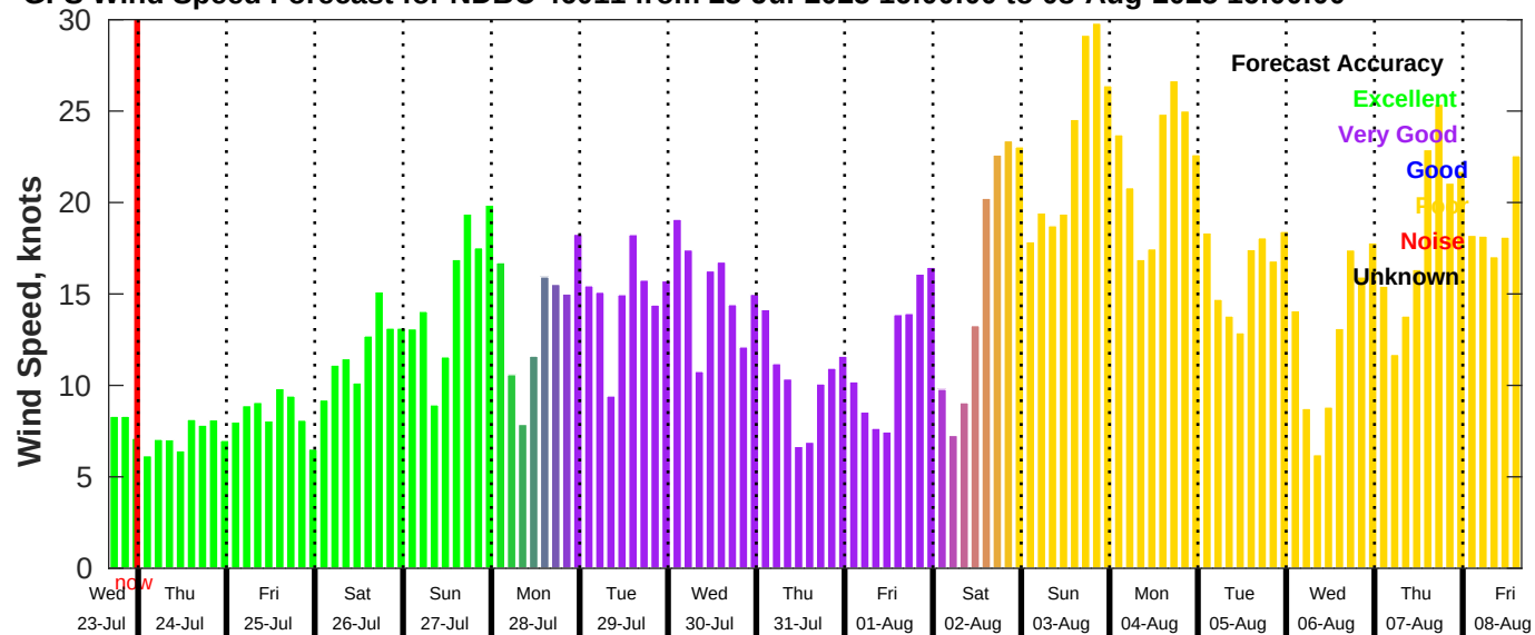
GFS Wind Speed Forecast for NDBC 46011 from 23-Jul-2025 16:00:00 to 08-Aug-2025 16:00:00
