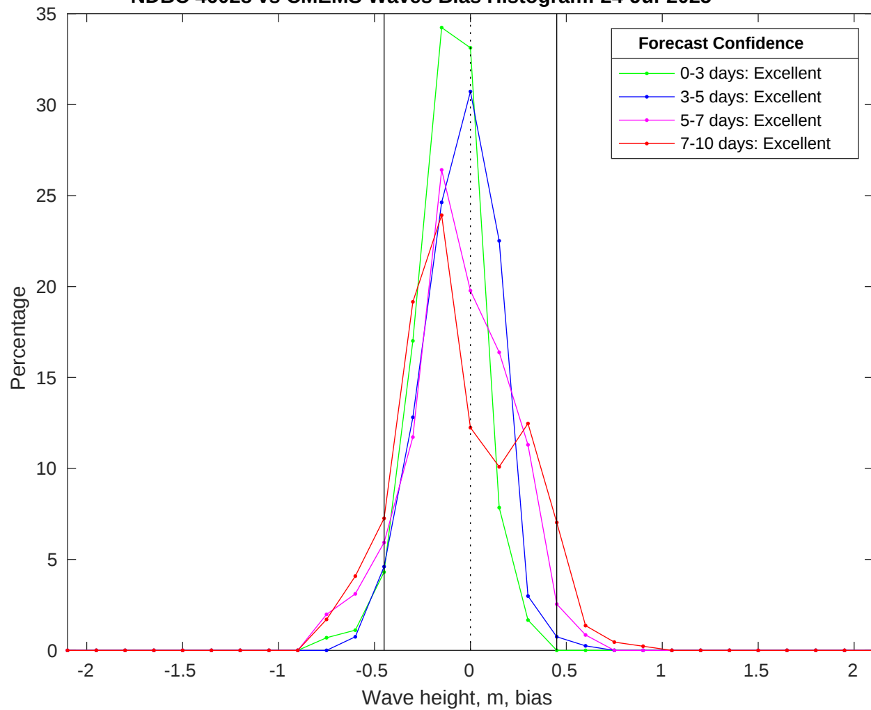
NDBC 46028 vs CMEMS Waves Bias Histogram: 24-Jul-2025
