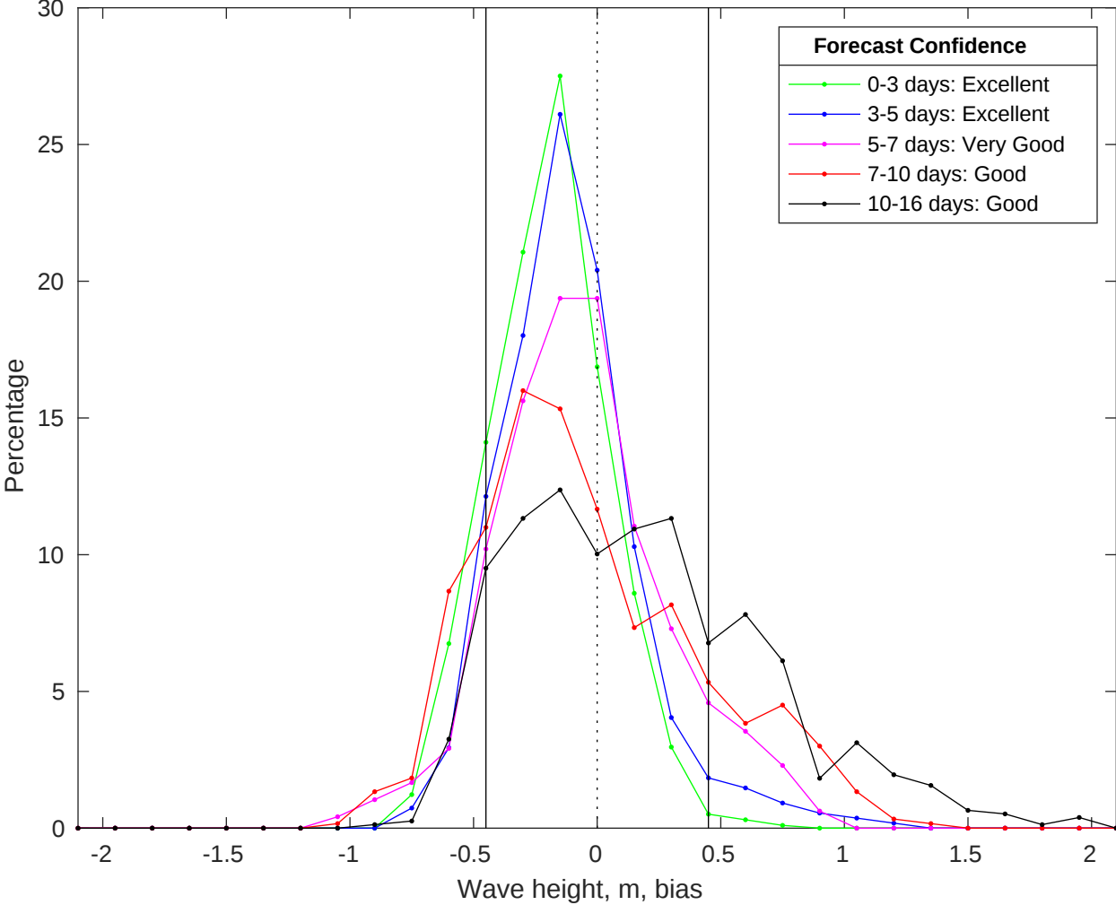
NDBC 46028 vs GFS Waves Bias Histogram: 24-Jul-2025
