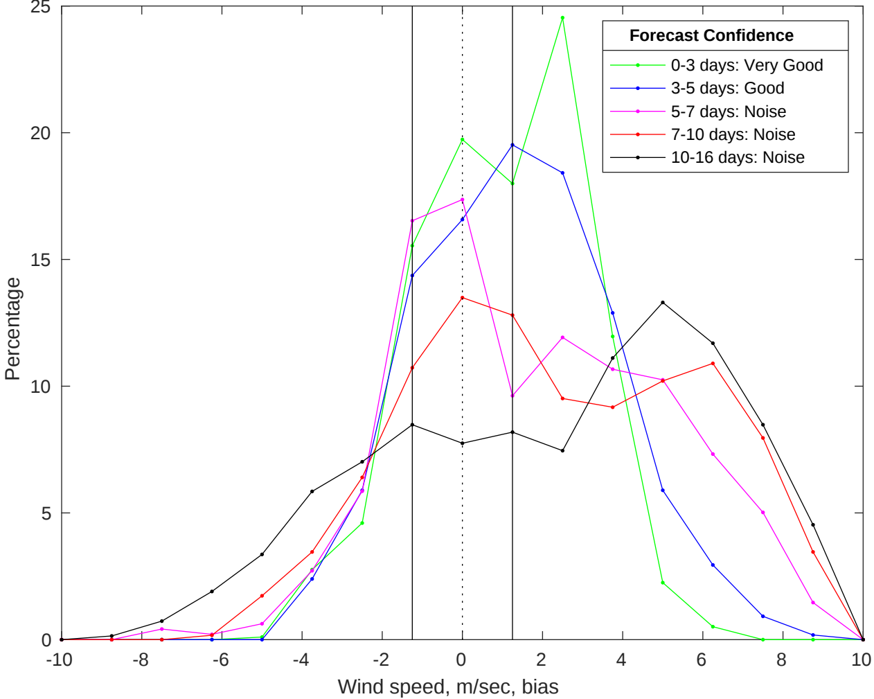
NDBC 46028 vs GFS Winds Bias Histogram: 24-Jul-2025
