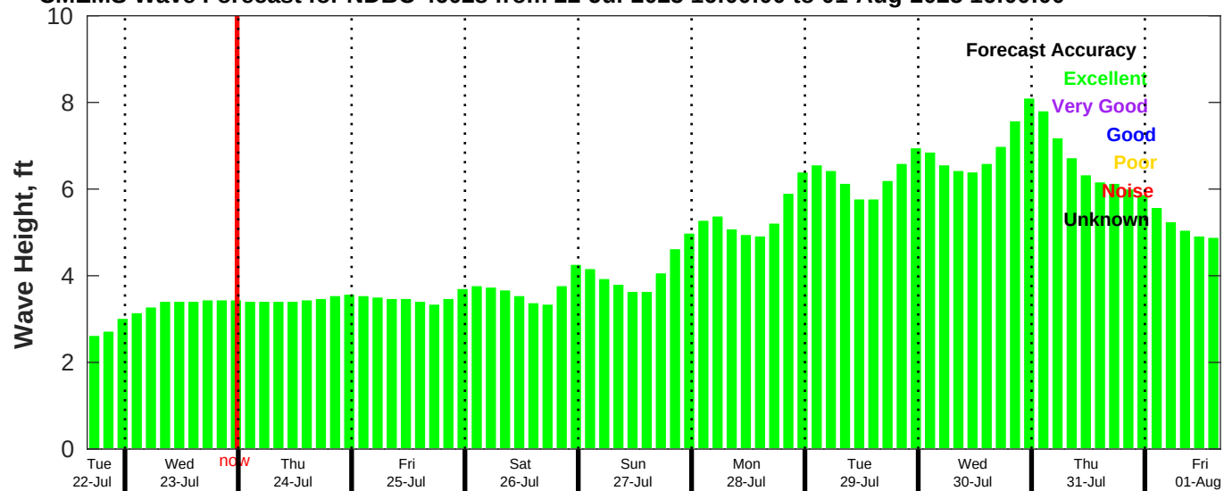
CMEMS Wave Forecast for NDBC 46028 from 22-Jul-2025 16:00:00 to 01-Aug-2025 16:00:00
