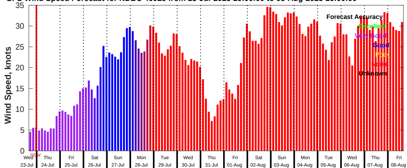
GFS Wind Speed Forecast for NDBC 46028 from 23-Jul-2025 16:00:00 to 08-Aug-2025 16:00:00
