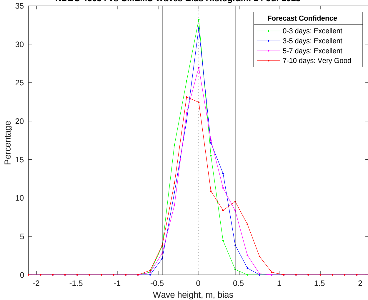
NDBC 46054 vs CMEMS Waves Bias Histogram: 24-Jul-2025
