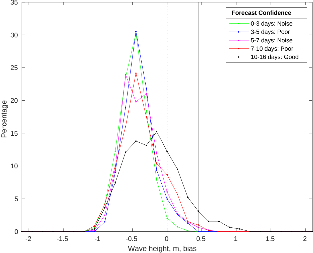
NDBC 46054 vs GFS Waves Bias Histogram: 24-Jul-2025
