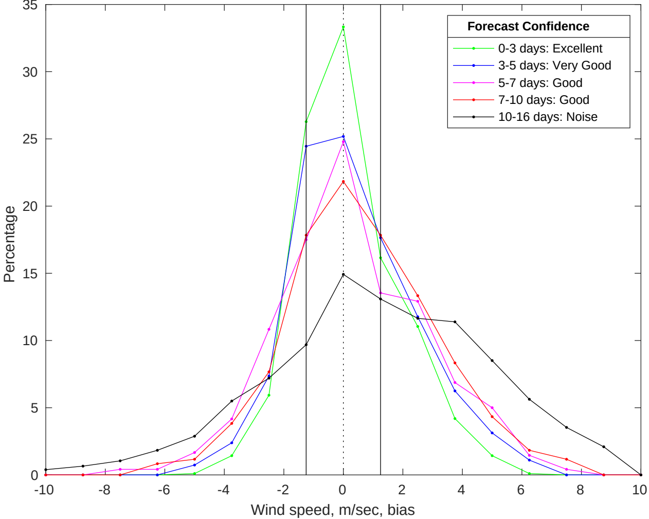
NDBC 46054 vs GFS Winds Bias Histogram: 24-Jul-2025
