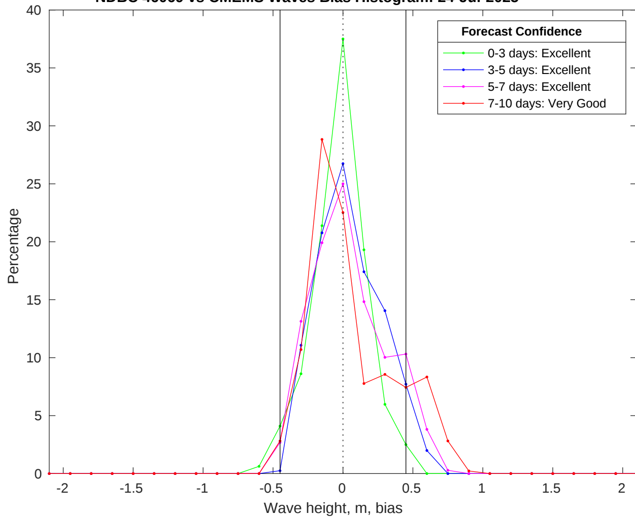
NDBC 46069 vs CMEMS Waves Bias Histogram: 24-Jul-2025
