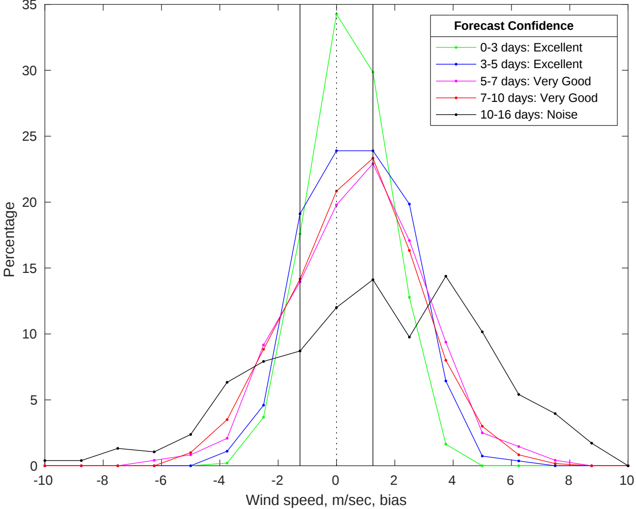
NDBC 46069 vs GFS Winds Bias Histogram: 24-Jul-2025
