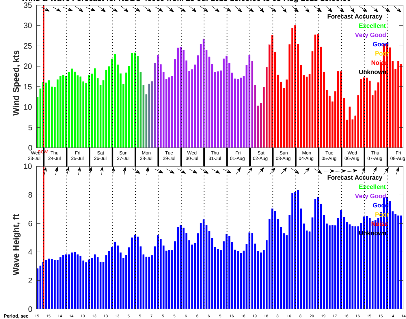
Wind & Wave Forecast for NDBC 46069 from 23-Jul-2025 16:00:00 to 08-Aug-2025 16:00:00
