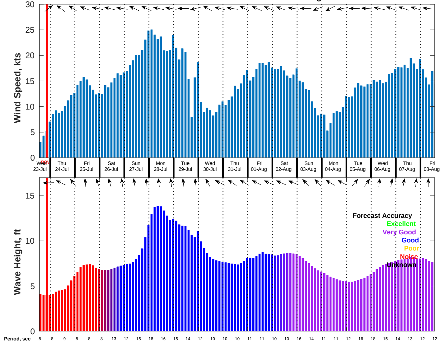
Wind & Wave Forecast for NDBC 51209 from 23-Jul-2025 13:00:00 to 08-Aug-2025 13:00:00
