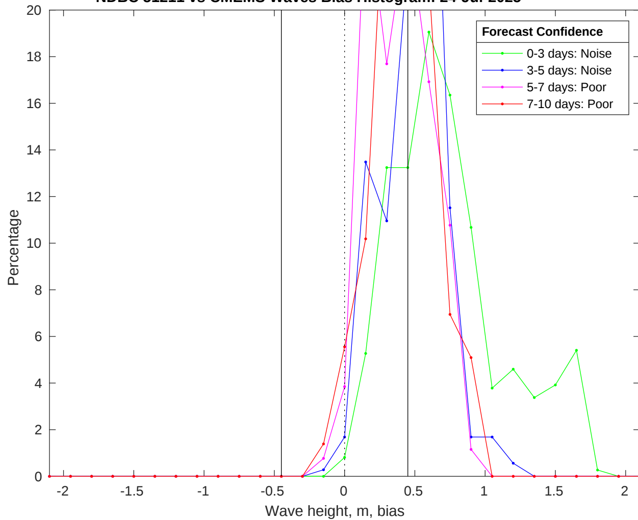
NDBC 51211 vs CMEMS Waves Bias Histogram: 24-Jul-2025
